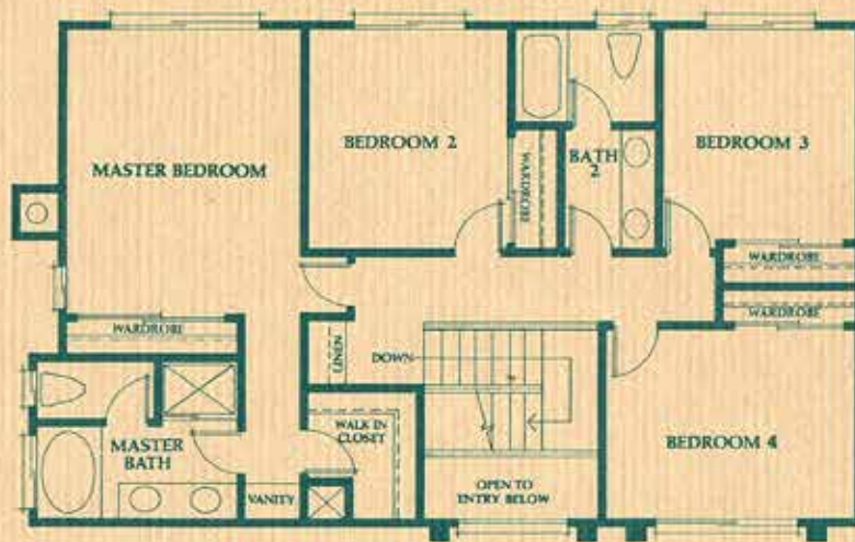
SECOND FLOOR
