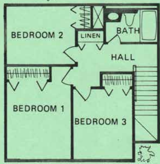
PLAN 540 3 BEDROOM
