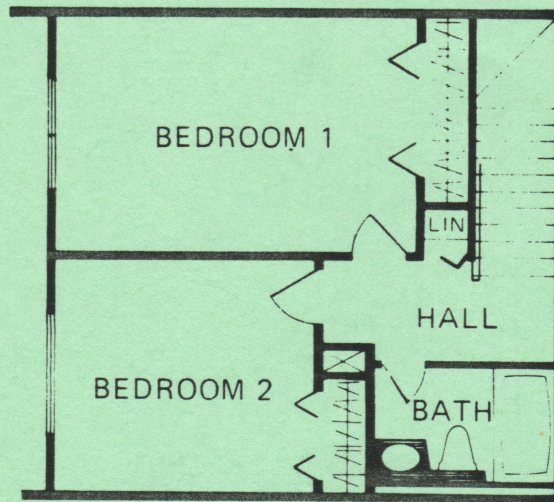
PLAN 541 2 BEDROOM
